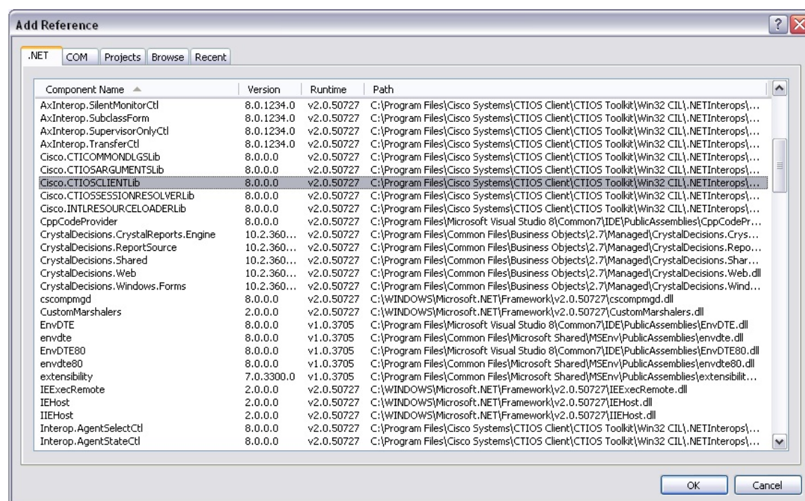
Figure 10: CTI OS COM CIL RCWs References Needed for Visual Basic .NET COM Programming
