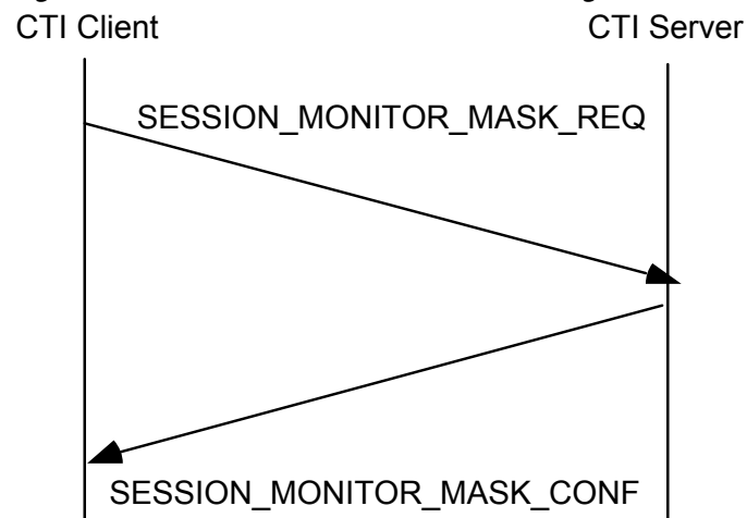
Figure 5-5 Session Monitor Start Message Flow
